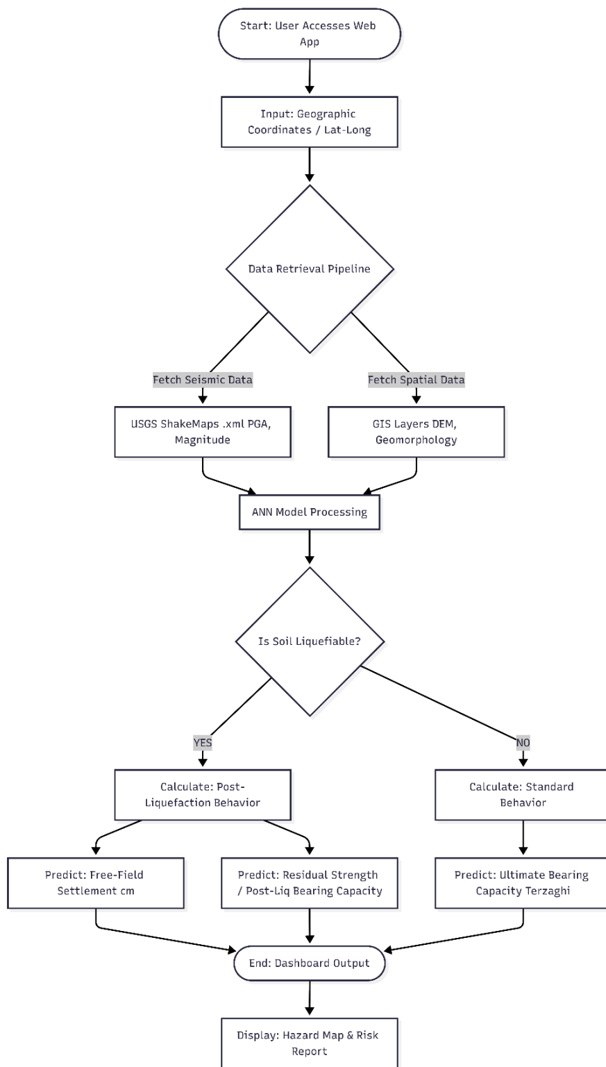
Flowchart of Web-Based Liquefaction Prediction System (Tarlac Province)
